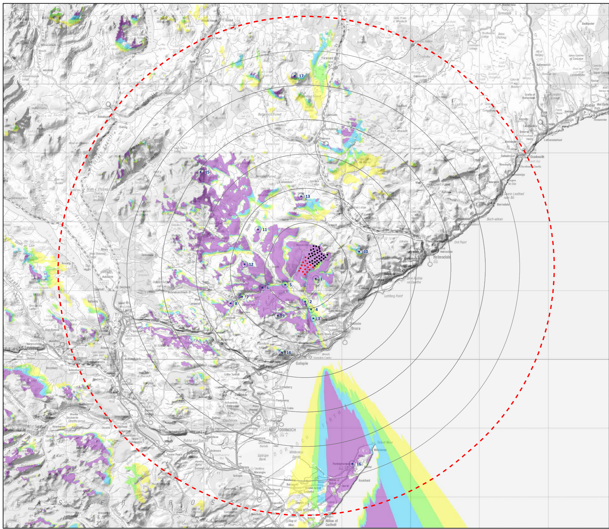
Figure 7.8a BLADE TIP ZTV WITH VIEWPOINTS Gordonbush Extension Wind Farm Environmental Statement
