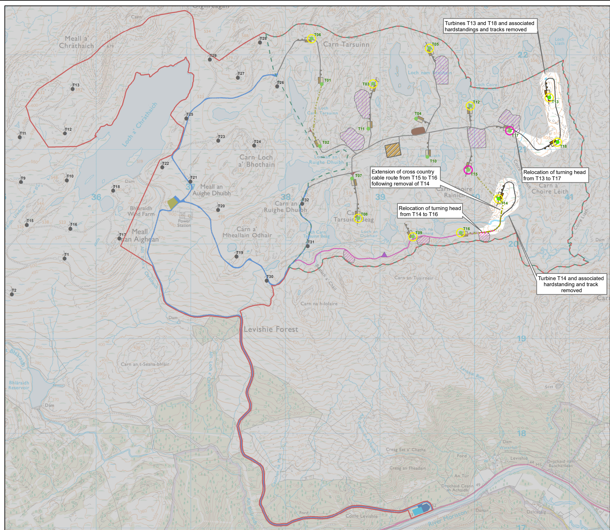
Figure 2.1 Site Layout Plan - Proposed Changes Bhlaraidh Wind Farm Extension Additional Information Report
